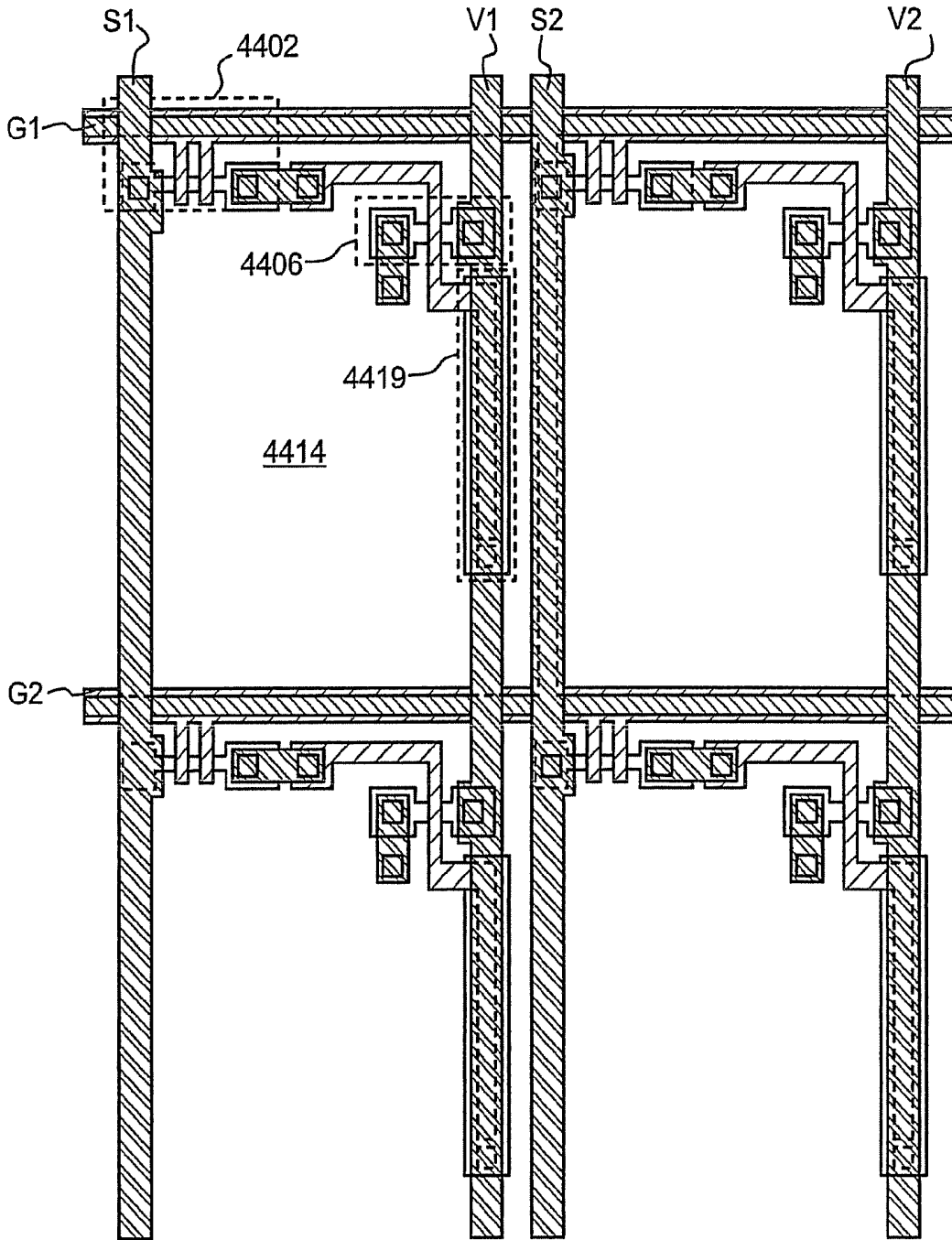
FIG. 41 PRIOR ART
